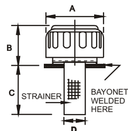
WELD TYPE
