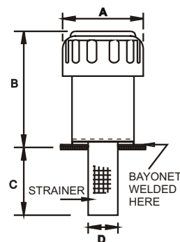
FSBW - 25 HN
