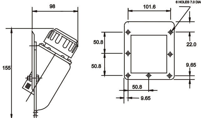
FSB - 25 BM
