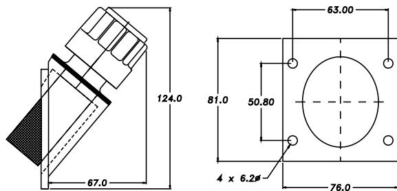
FSB - 05 BM
